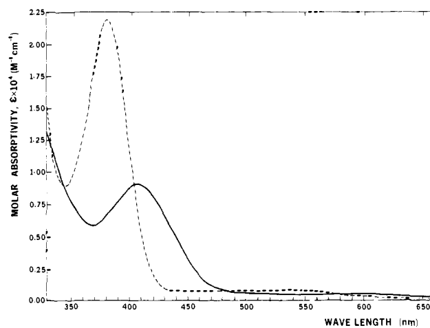
Figure 2. Electronic spectra of the Cu(II) and Cu(III) dithiooxalate complexes in \text{CH}_2\text{Cl}_2 at 25 °C: (—) (\text{BzPh}_3\text{P})_2\text{Cu}(\text{Dto})_2 ; (---) (\text{BzPh}_3\text{P})\text{Cu}(\text{Dto})_2 .
