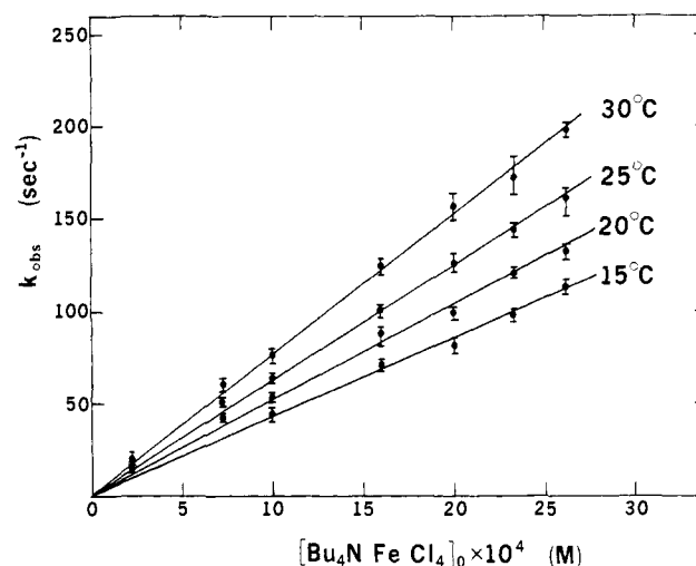
Figure 3. Rate constant for the (\text{Bu}_4\text{N})_2\text{Cu}(\text{Dto})_2-(\text{Bu}_4\text{N})\text{FeCl}_4 reaction as a function of [(\text{Bu}_4\text{N})\text{FeCl}_4] in 0.1 M \text{Bu}_4\text{NCl} at various temperatures.
