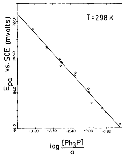
Figure 5. Variation in the E_{pa} values for \text{Cu}(\text{S}_2\text{C}_2\text{O}_2)_2^{2-} as a function of \log ([\text{Ph}_3\text{P}]/a) at 24 °C in the \text{CH}_2\text{Cl}_2 .
